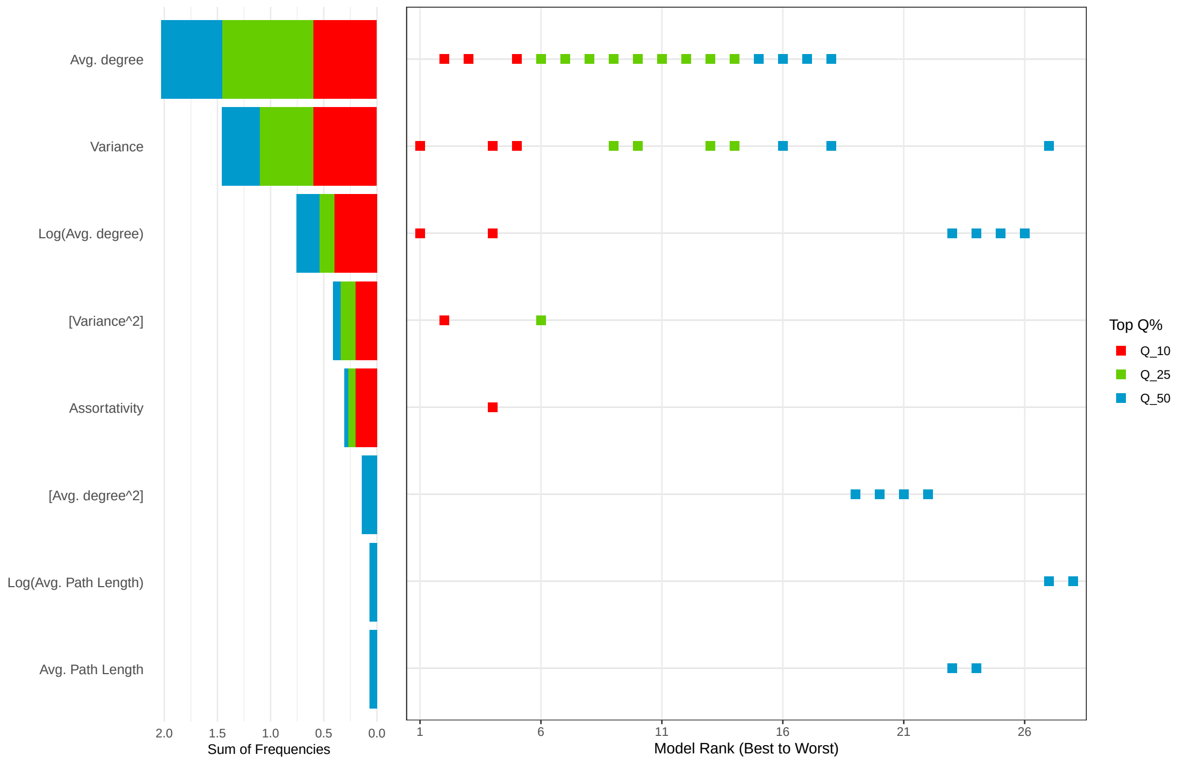
Model Stability Matrix: Generation Time
